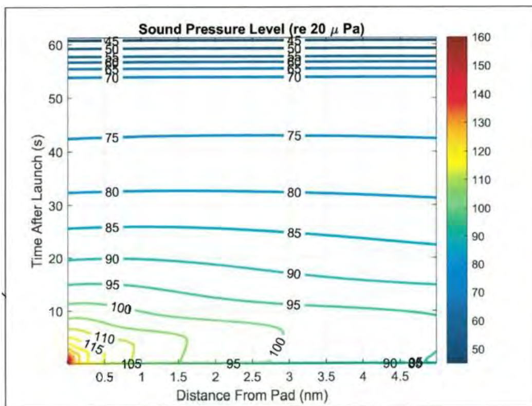
Figure 11. Modeled maximum sound pressure levels at various distances (nautical miles) from the launch pad and duration for launches during Joint Flight Campaign activities.
